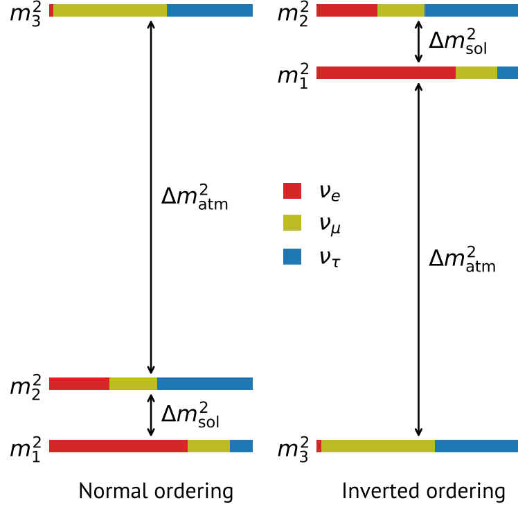
Figure 2.2: The two possible neutrino mass ordering scenarios allowed by current neutrino oscillation data, with the solar neutrino mass squared difference defined as \Delta m_{\text{sol}}^2 \equiv \Delta m_{21}^2 and the atmospheric neutrino mass squared difference defined as \Delta m_{\text{atm}}^2 \equiv \Delta m_{32}^2 \approx \Delta m_{31}^2 .
