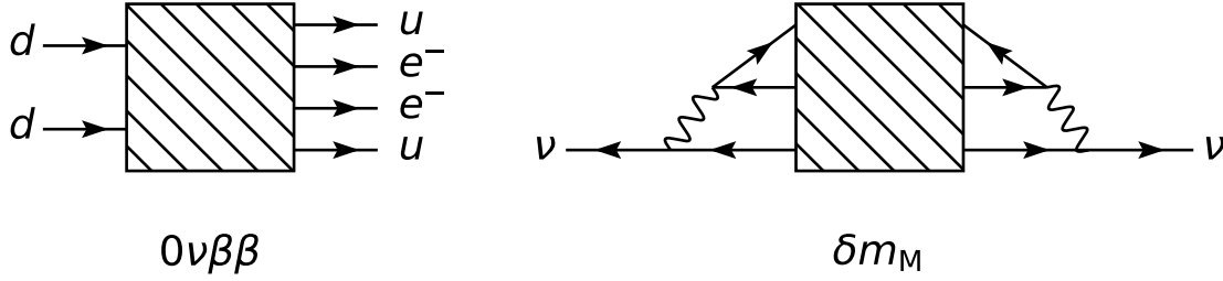
Figure 2.9: The operator which causes 0\nu\beta\beta (left) need not involve Majorana neutrinos. By crossing symmetry, however, if such an operator exists, it would contribute an effective Majorana mass for neutrinos at the four-loop level (right), enabling particles to oscillate into antiparticles and vice versa. This result is known as the Black Box Theorem.
